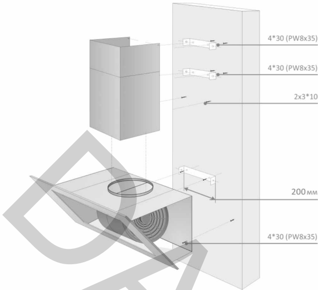
Fig. 8 Cooker hood installation scheme
